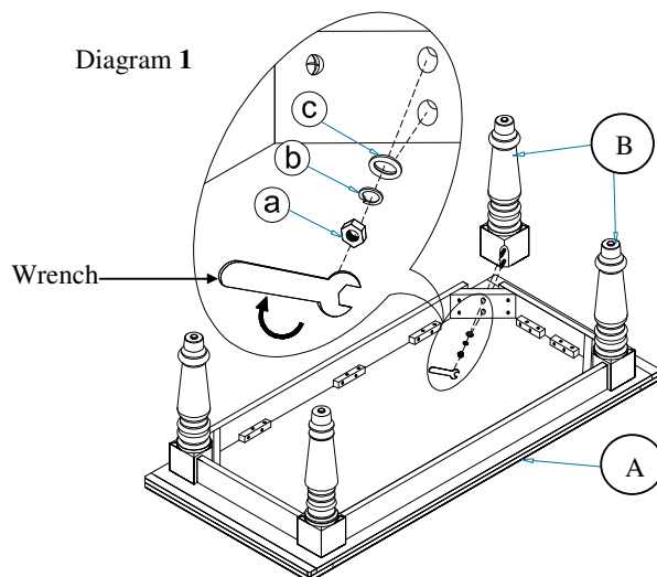
Adjustable Leveler
